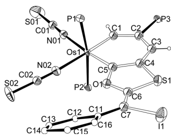
Figure 1. X-ray structure of complex 2A (ellipsoids set at 50% probability). Phenyl rings in \text{PPh}_3 groups and some of the hydrogen atoms are omitted for clarity.
