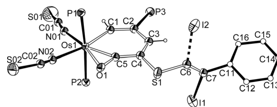
Figure 2. X-ray structure of complex 3 (ellipsoids set at 50% probability). Phenyl rings in \text{PPh}_3 groups, some of the hydrogen atoms, and the counteranion are omitted for clarity. Selected bond distances [ \text{\AA} ] and angles [ ^\circ ]: Os–C1 2.061(9), Os–C5 1.971(9), Os1–O1 2.159(6), C1–C2 1.361(14), C2–C3 1.415(14), C3–C4 1.344(15), C4–C5 1.398(14), C5–O1 1.229(12), C4–S1 1.768(10), C6–S1 1.713(14), C6–C7 1.17(2), C7–C11 1.55(2), C7–I1 2.098(17), C6–I2 2.362(19); C1–Os1–C5 78.8(4), Os1–C1–C2 133.4(7), C1–C2–C3 124.1(9), C2–C3–C4 123.5(9), C3–C4–C5 117.9(9), C4–C5–Os1 142.3(8), C5–O1–Os1 64.5(5), O1–C5–Os1 81.3(6), C5–Os1–O1 34.2(3), C6–S1–C4 101.5(6), C7–C6–S1 136.9(17).
